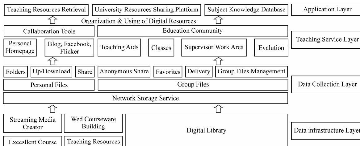
Fig. 1 Architecture of the E-learning platform
